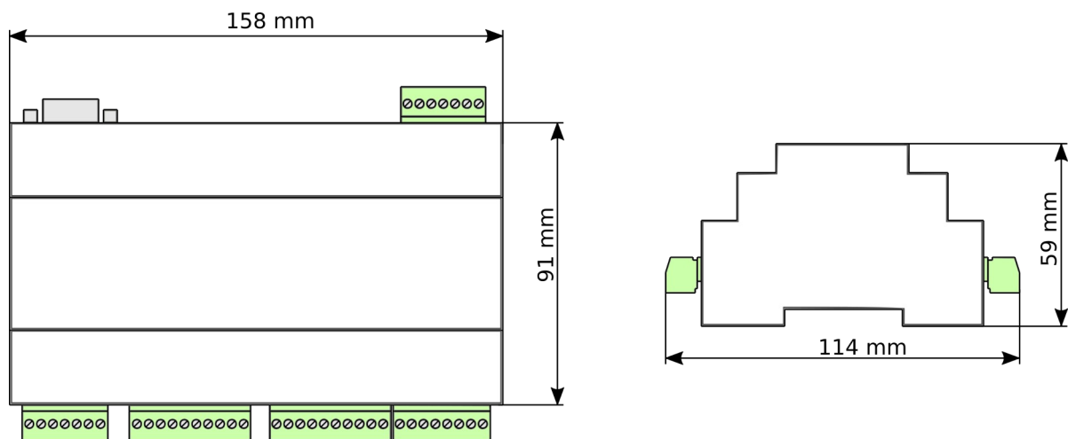
Fig. 5. RB350-CM3 dimensions
