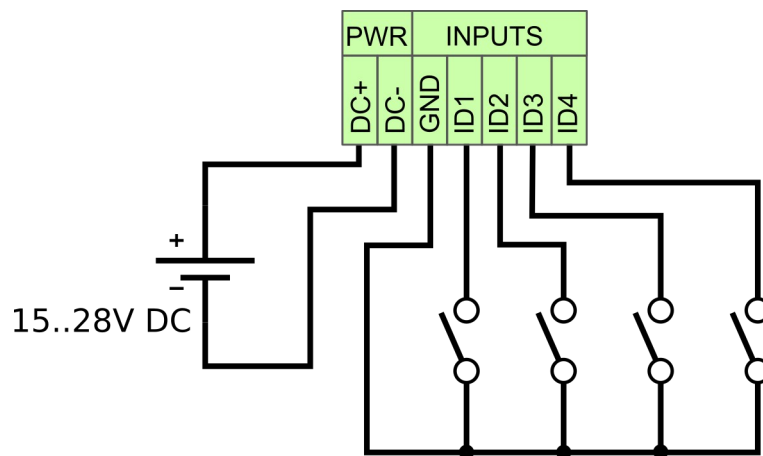
Fig. 1. Power supply and dry contact inputs connections
