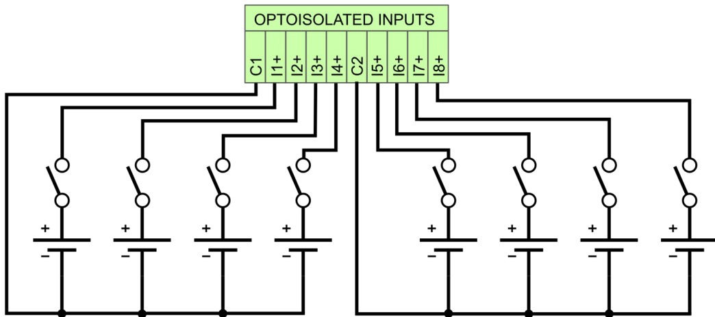
Fig. 2. Digital opto-isolated inputs connections
